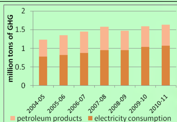
Figure 4.4b: Emissions from electricity consumption and vehicular emissions petroleum products
