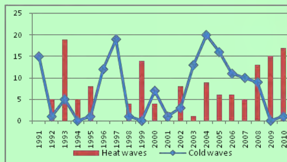
Figure 6.3: Frequency of heat and cold waves in Chandigarh in the last 20 years
