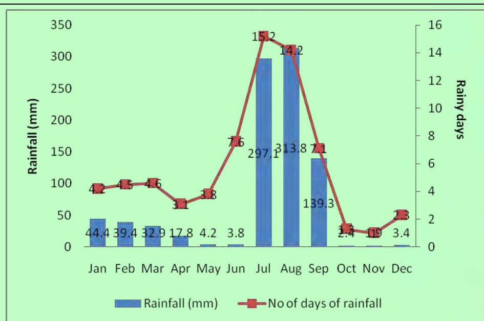
Figure 1.2 Rainfall and number of rainy days in Chandigarh (Source: Air Force Climate Data from 1970-2005)
