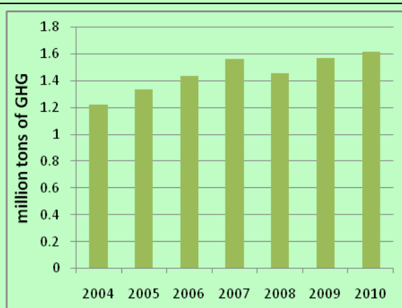
Figure 4.4a: Total emissions in Chandigarh UT.
